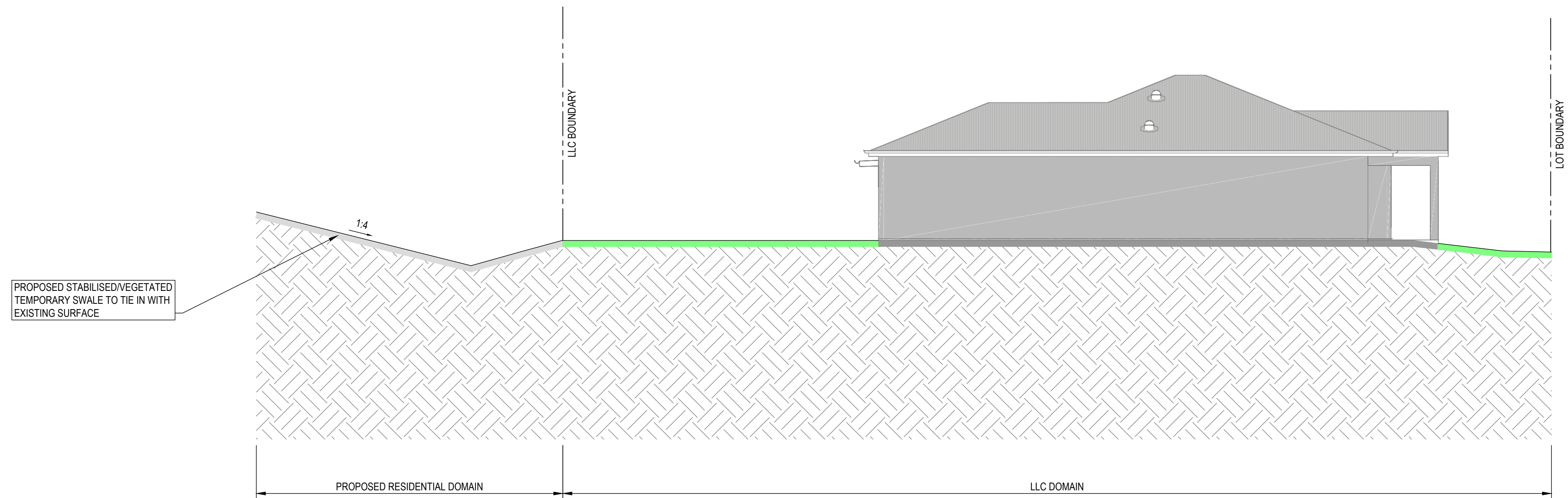
NORTHERN LOT INTERFACE TYPICAL SECTION 13 SCALE 1:100 SK040
